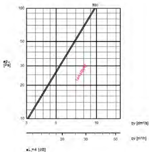
KWH, section 1000, static pressure loss and sound data
