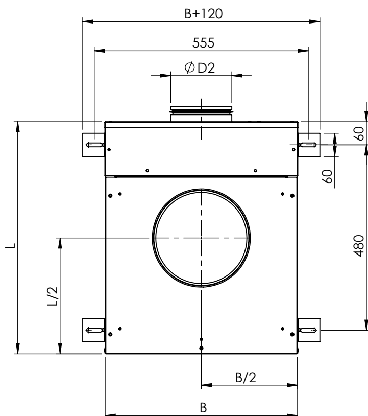
HMM DIMENSIONS, unit material thickness 0.5 mm
